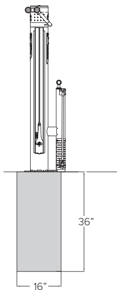
Footing 16" diameter X 36" depth
