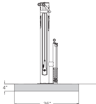
Slab 36" X 36" X 4" depth
